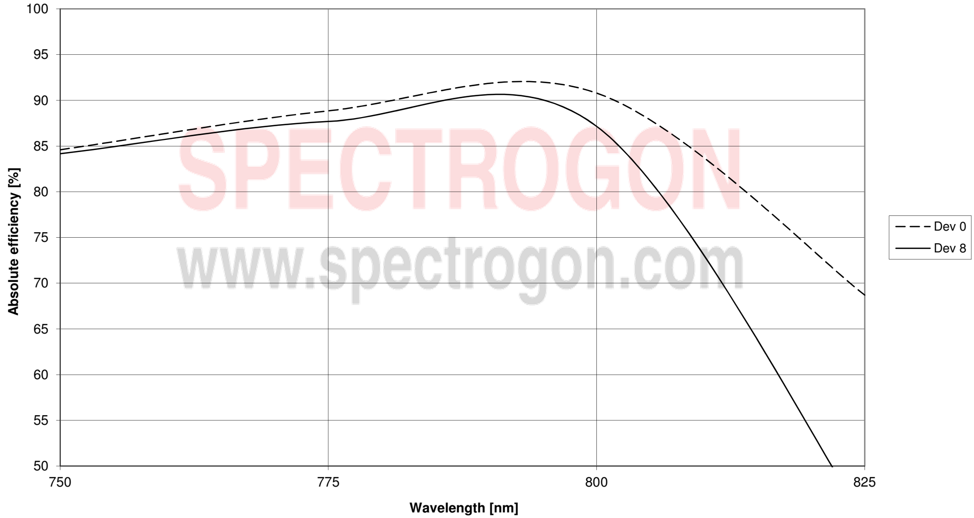
PC 2400, Expected efficiency (TM/-1) @ Dev 0 and 8 deg
