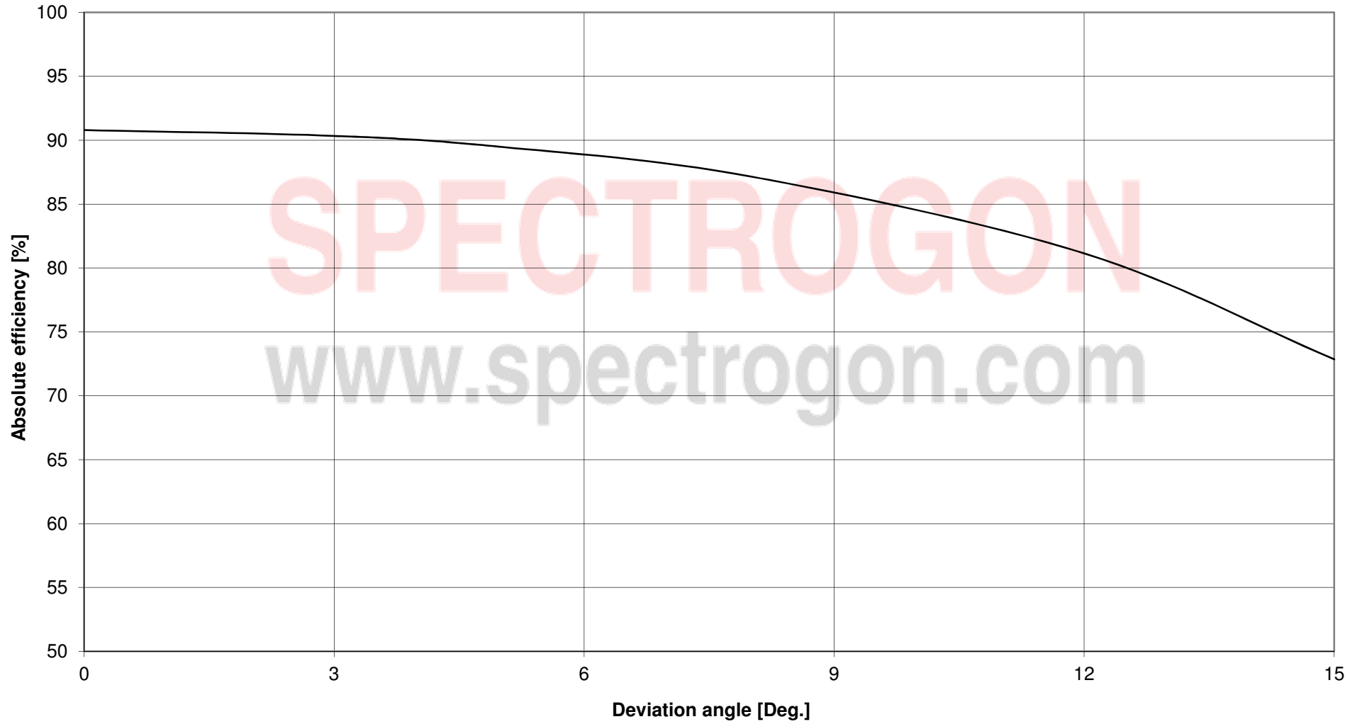
PC 2400, Expected efficiency (TM/-1) @ 800 nm
