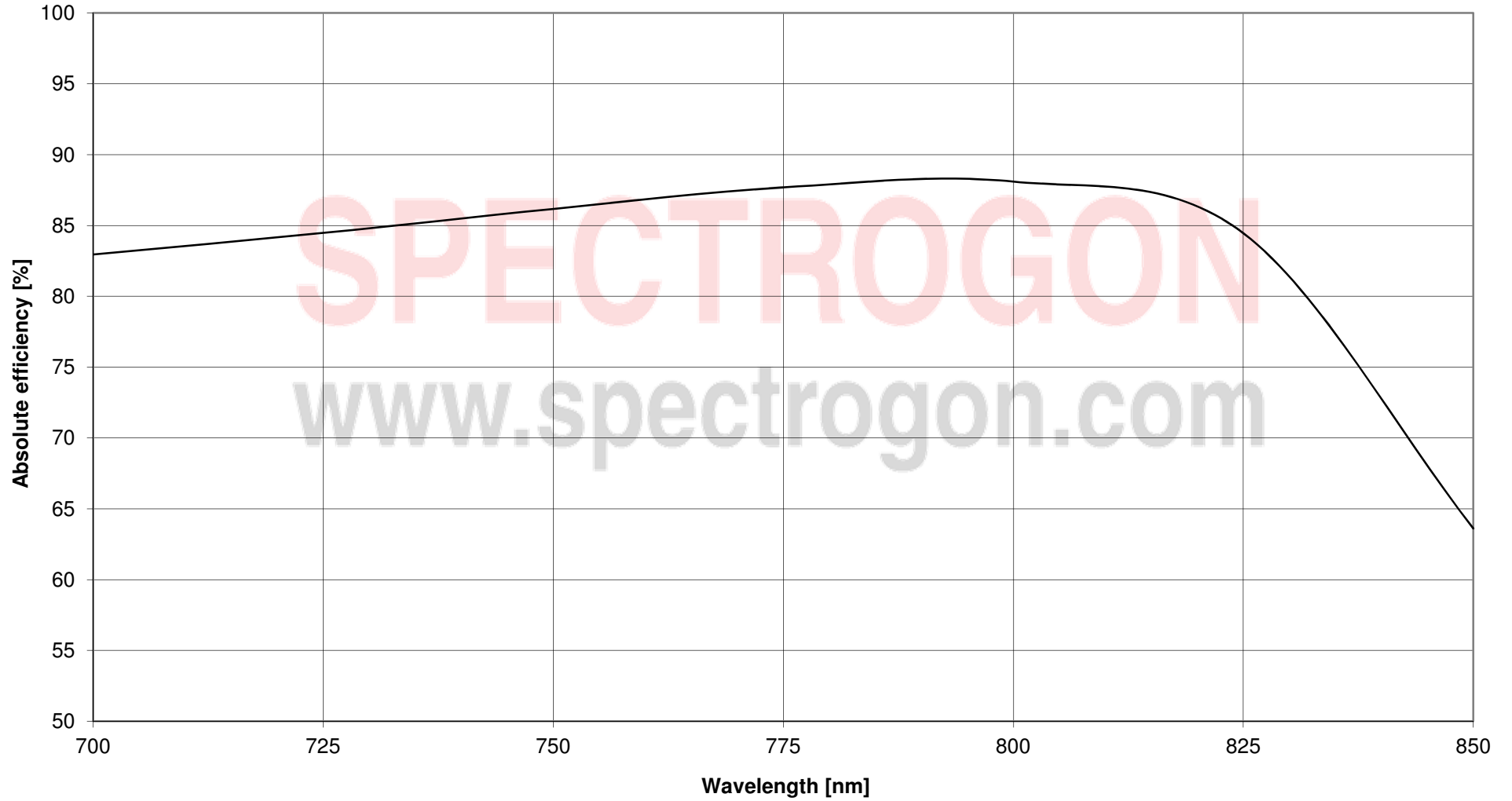
PC 2300, Expected efficiency (TM/-1) @ Dev 8 deg
