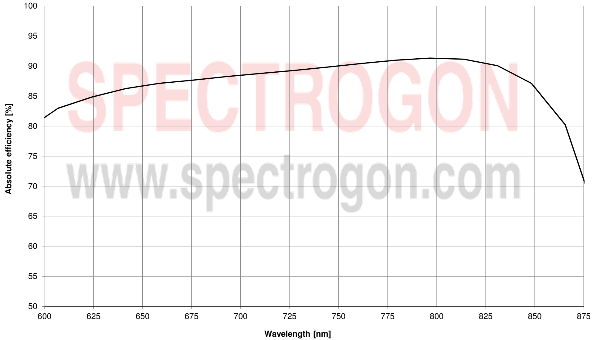
PC 2200, Expected efficiency (TM/-1) @ Dev 10°, Au
