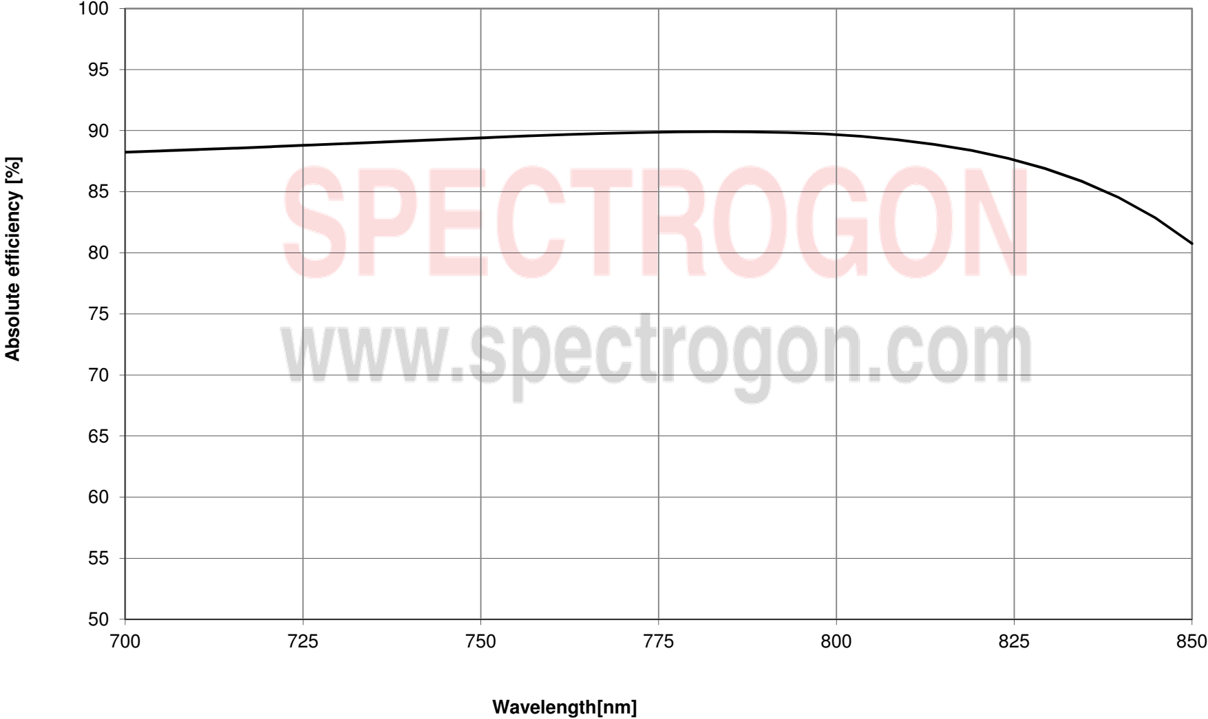
PC 2200, Expected efficiency (TM/-1) @ Dev 15°
