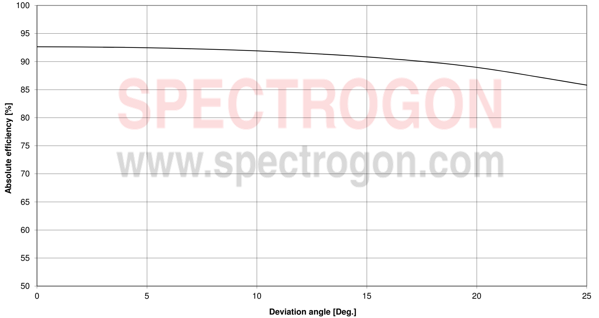
PC 2100, Expected efficiency (TM/-1) @ 800 nm
