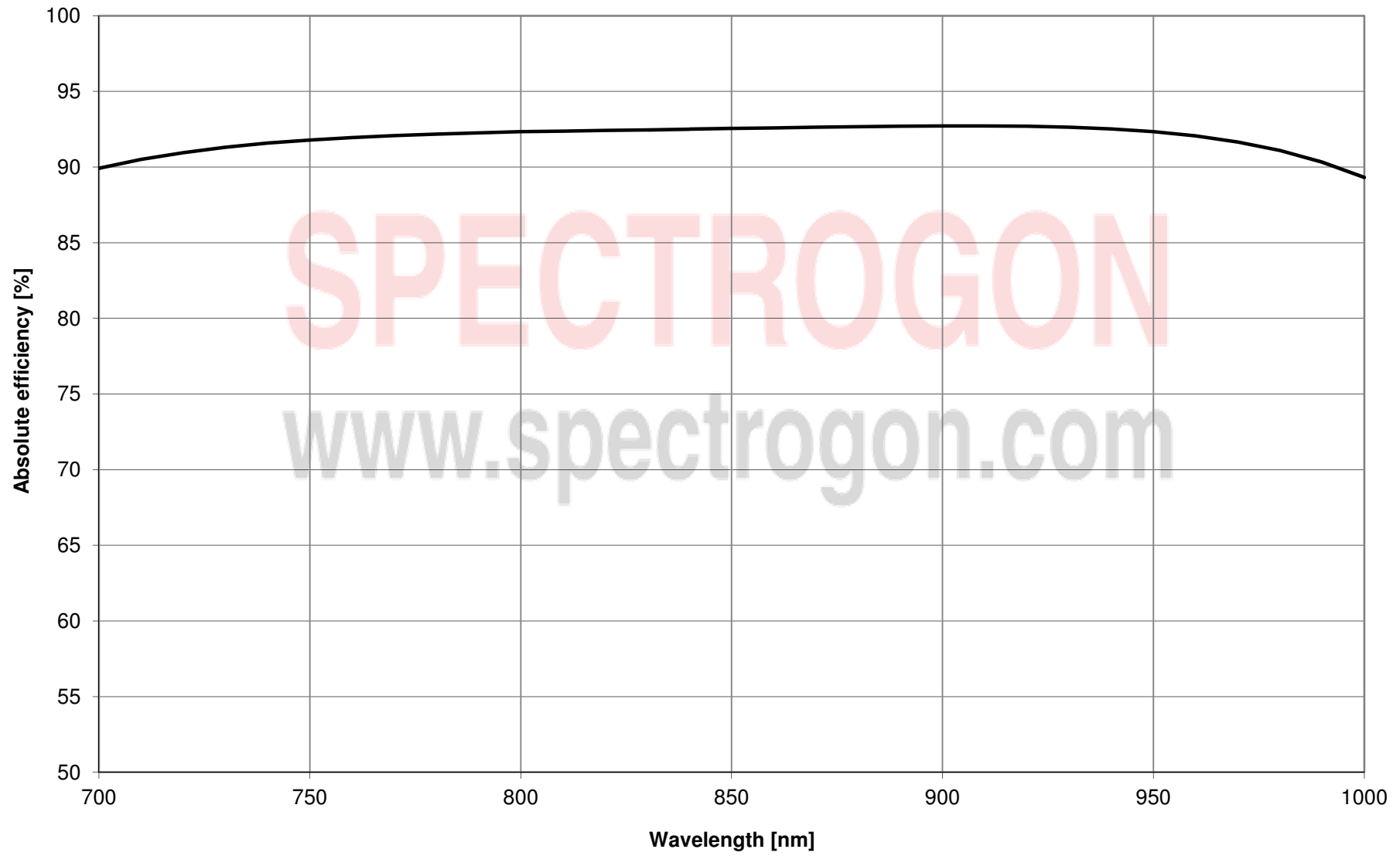
PC 1800, expected efficiency TM/-1 @Dev 10°, Au
