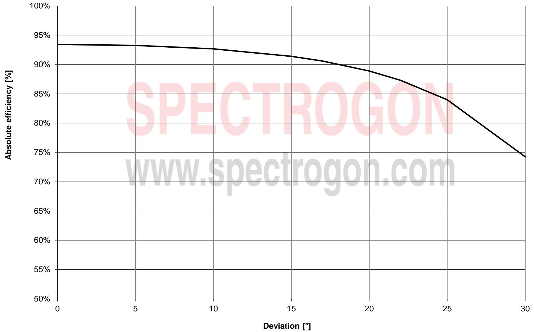
PC 1700 Expected efficiency (TM/-1) @ 1035 nm, Au
