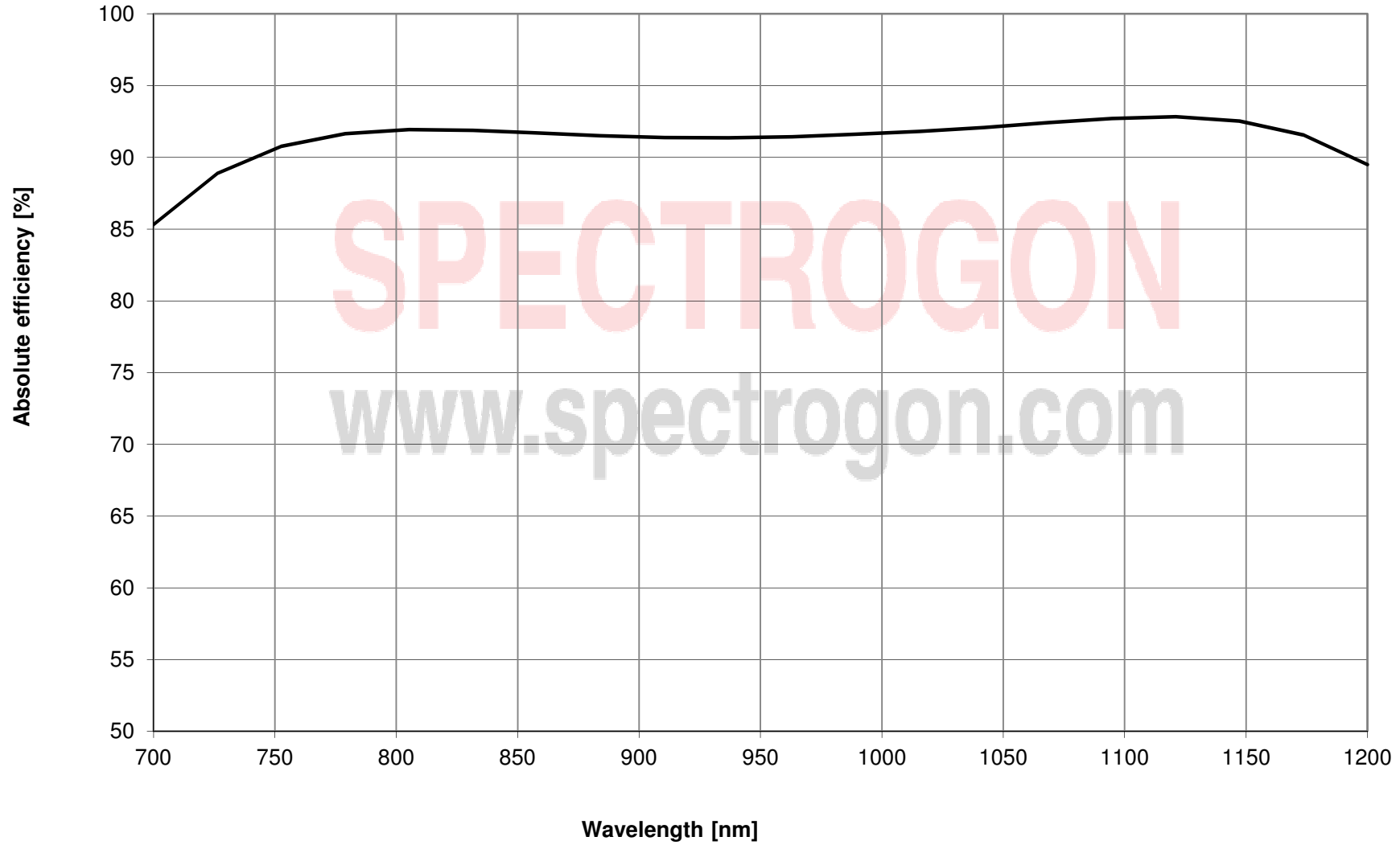
PC1500, Expected efficiency (TM/-1) @ Dev 13 deg
