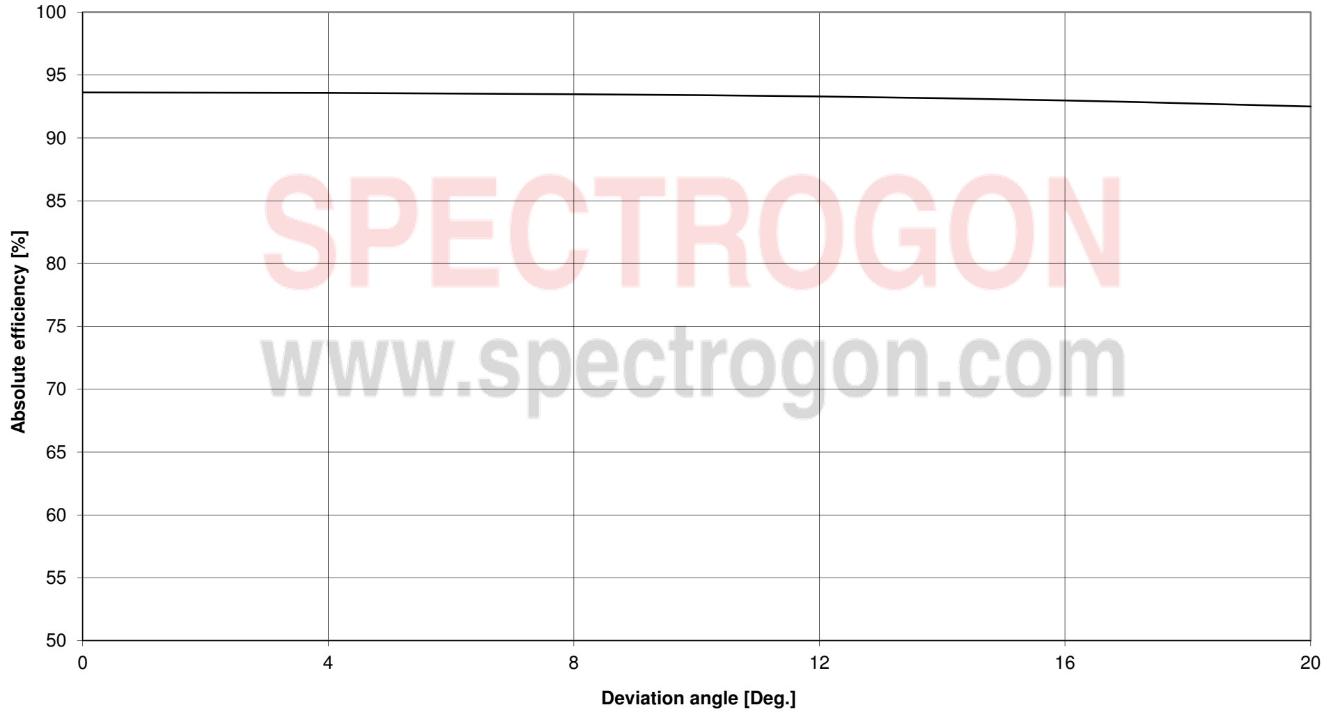
PC 1500, Expected efficiency (TM/-1) @ 1030 nm
