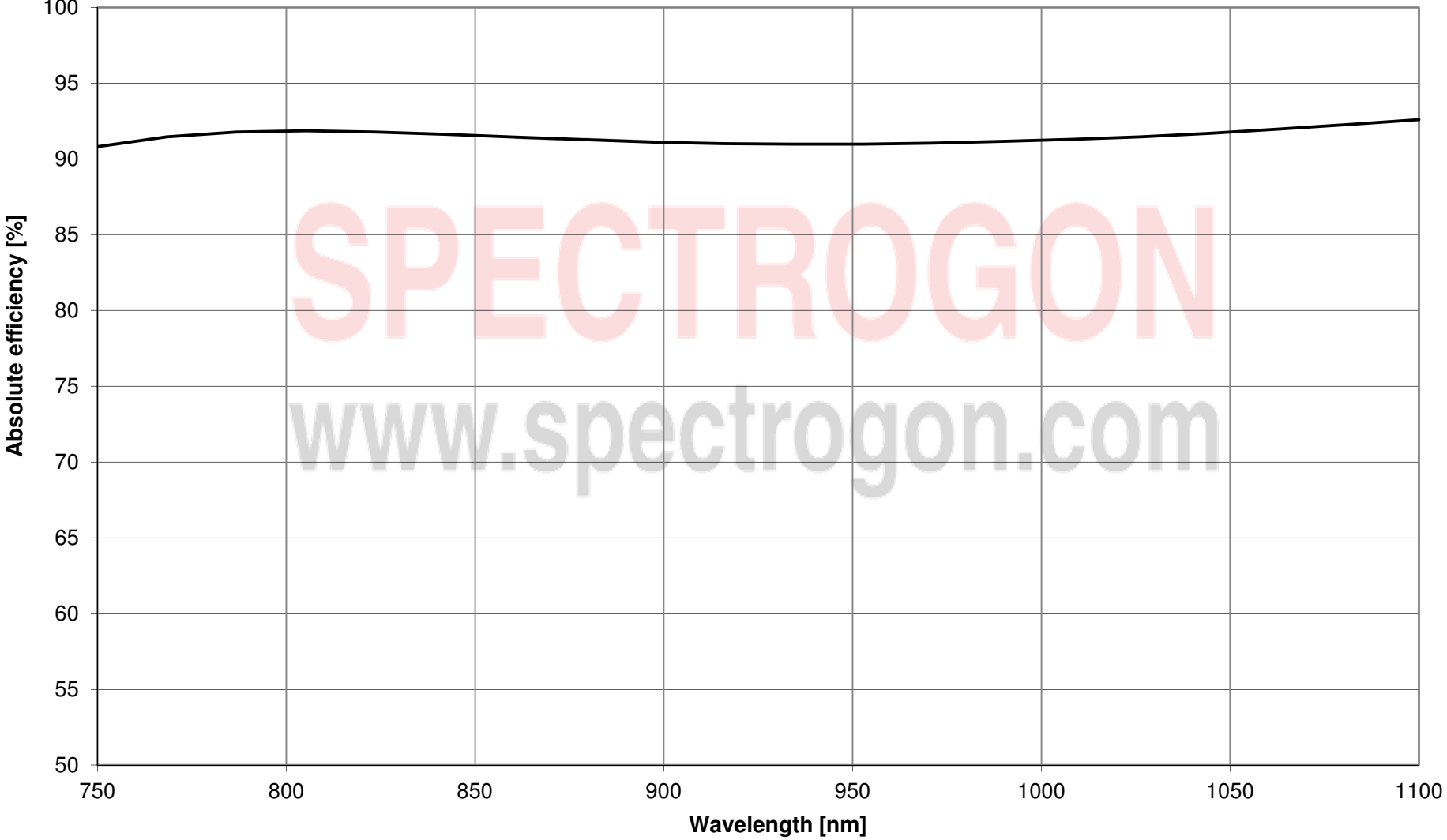
PC 1480, Expected efficiency (TM/-1) @ Dev 10
