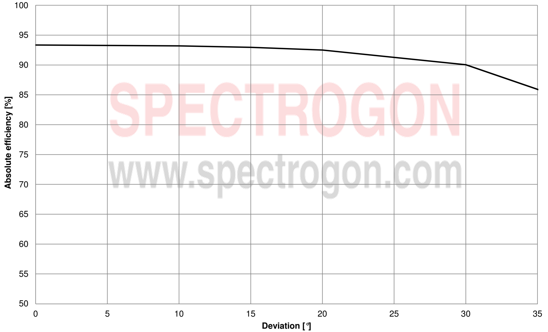
PC 1480 Expected efficiency (TM/-1) @1053nm, Au
