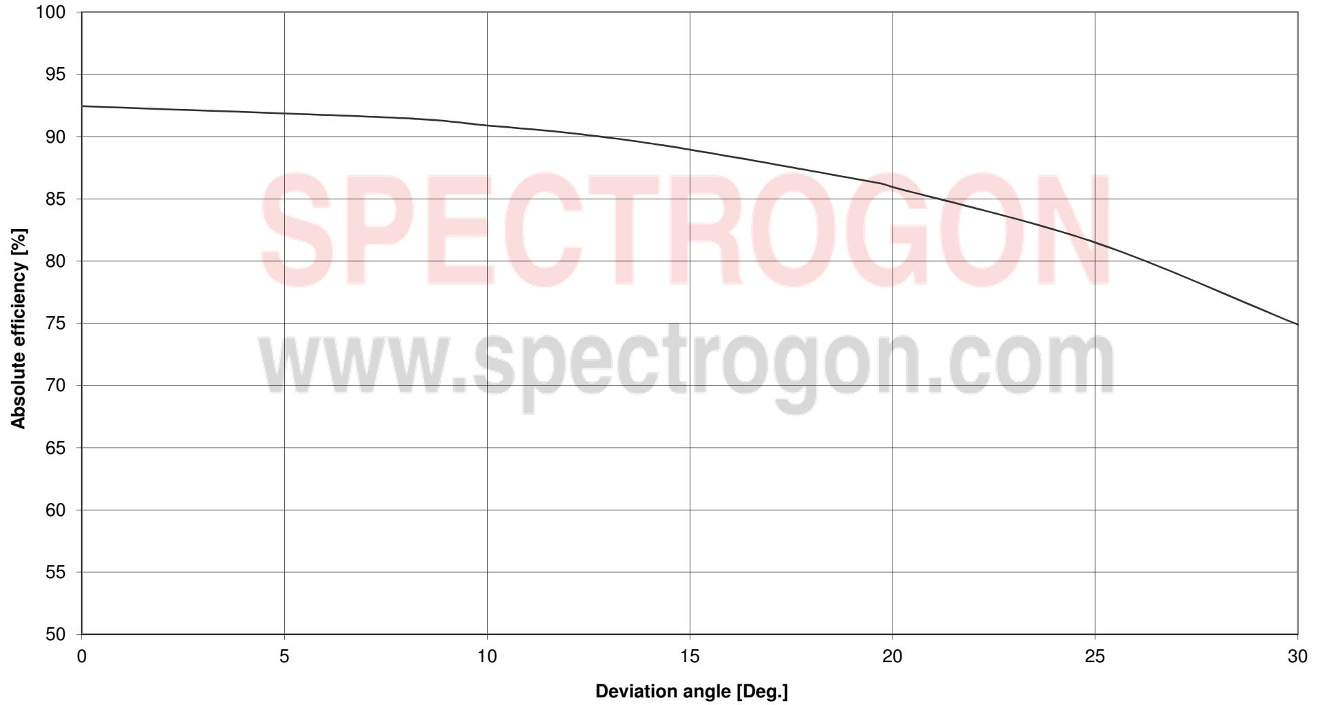
PC 1200, Expected efficiency (TM/-1) @ 800 nm
