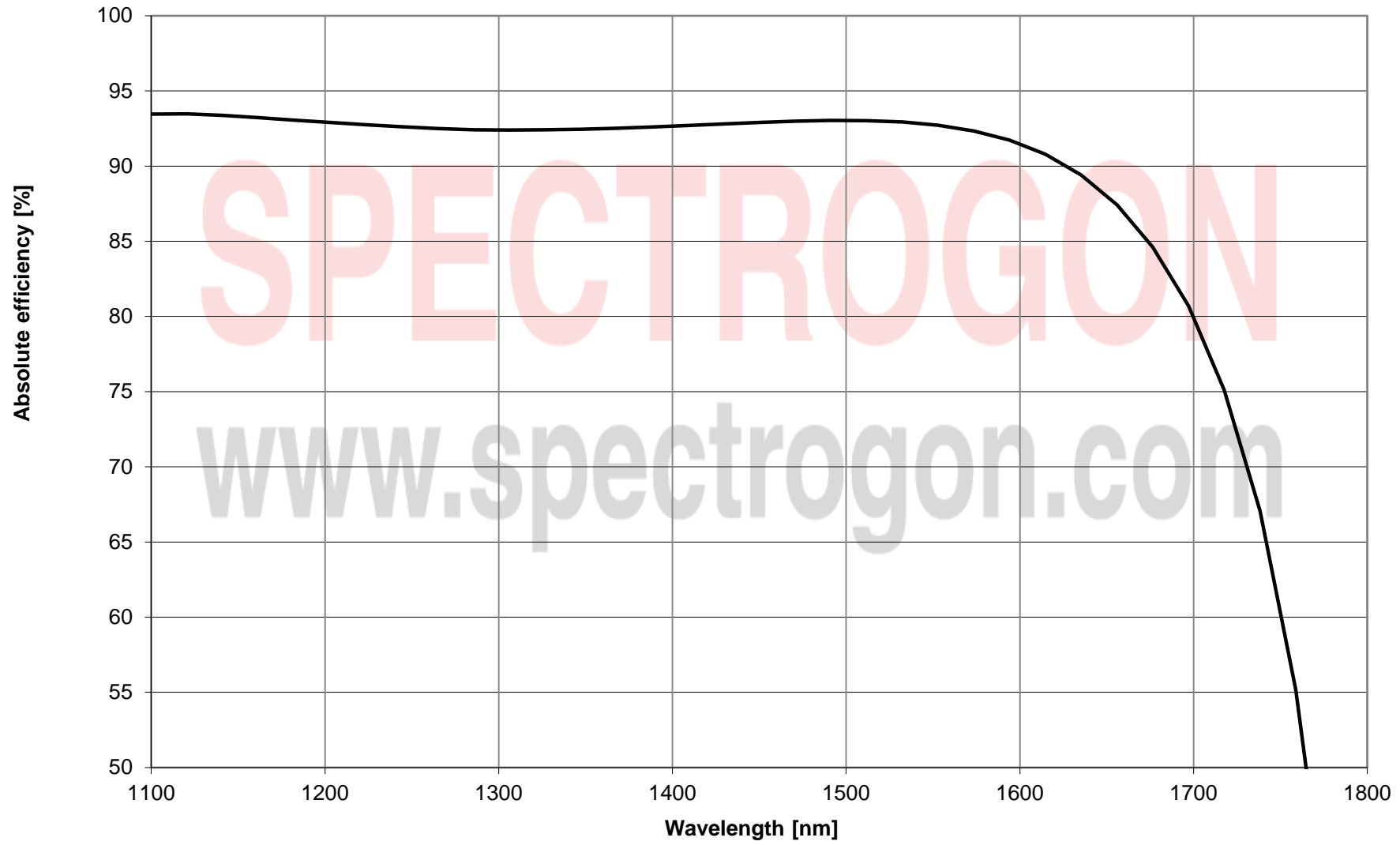
PC 1100 Expected efficiency (TM/-1)@ Dev 10°, Au
