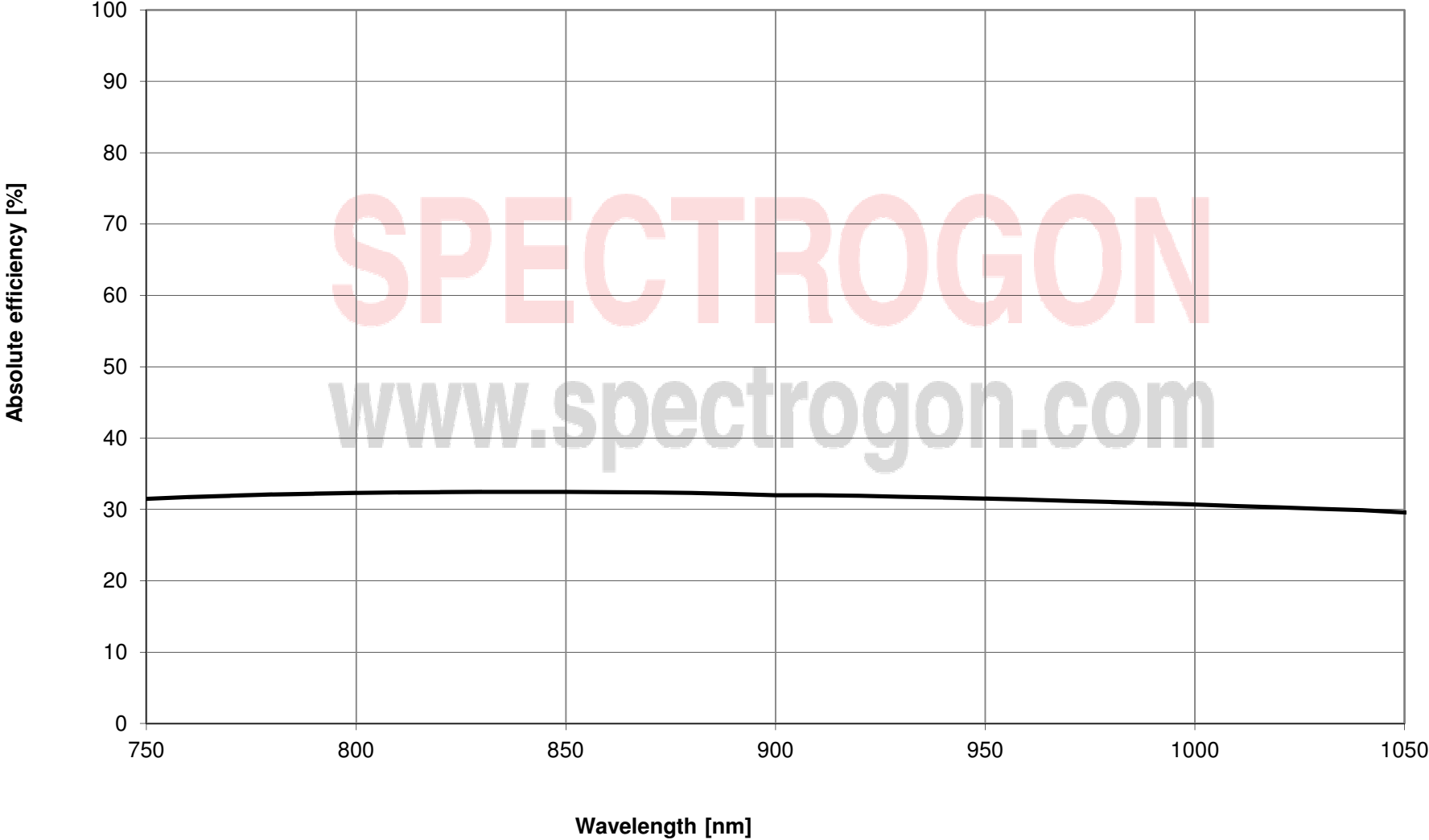
PC 0300, Expected efficiency (TM/-1) @ Dev 10°, Au
